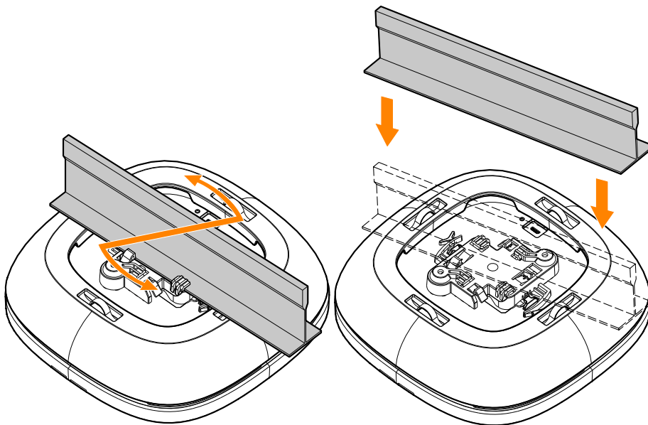
Figure 3 Removing the Access Point (with Sleeve) from a Ceiling Rail
