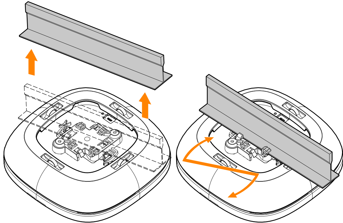
Figure 2 Installing the Access Point (with Sleeve) to a Ceiling Rail
